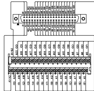
PCA7-4F40-TB34-M1-□
