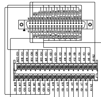
PCA7-4F40-TB34-M4
