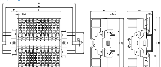
VTZL-4/4 VTZL-4/4-PE
