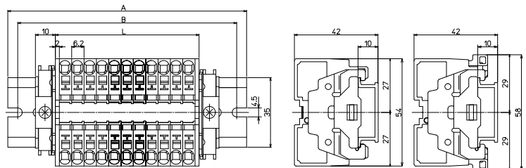
VTZL-4/2
