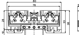
VTZ-2.5/4-PE
