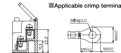
■ Applicable crimp terminal
